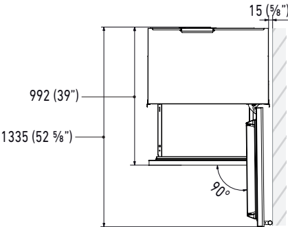
TOP VIEW, HINGE 90°
