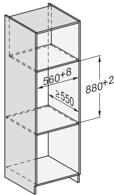
Installation DGC XXL, ESW7x20 installation drawings
