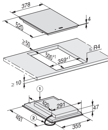
CS7612-1FL, CS7612FL, (installation drawing)
